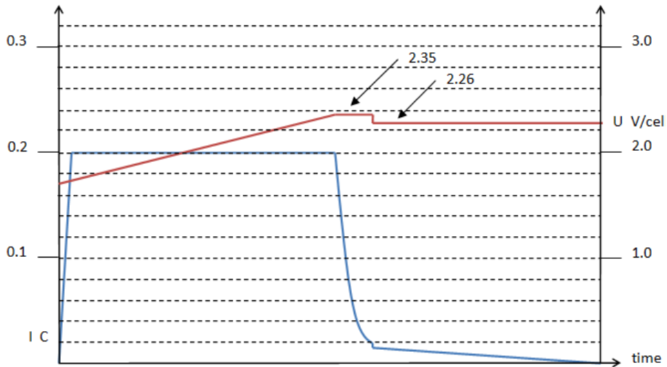
PP101 sealed (Temperature sensor supported)
