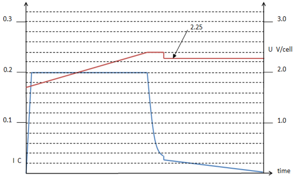
PP100 unsealed (Temperature sensor supported)
